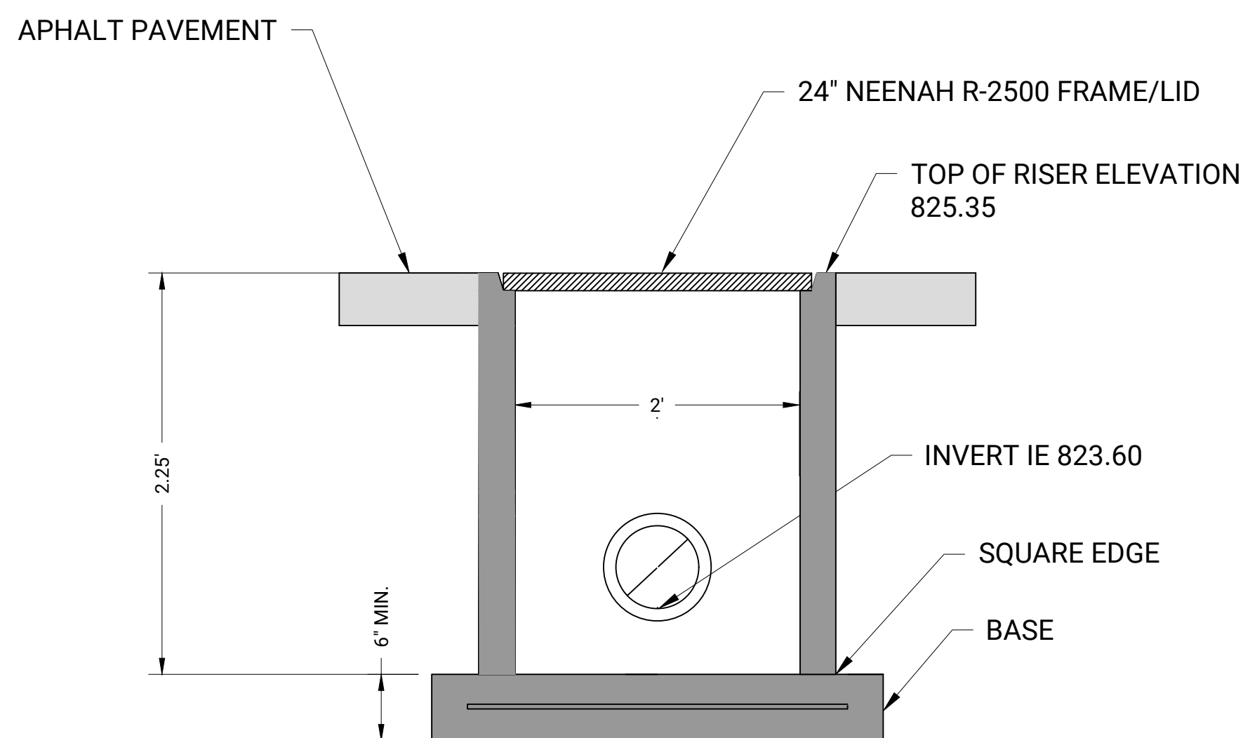
5 CATCH BASIN DETAIL C5.1 NOT TO SCALE
