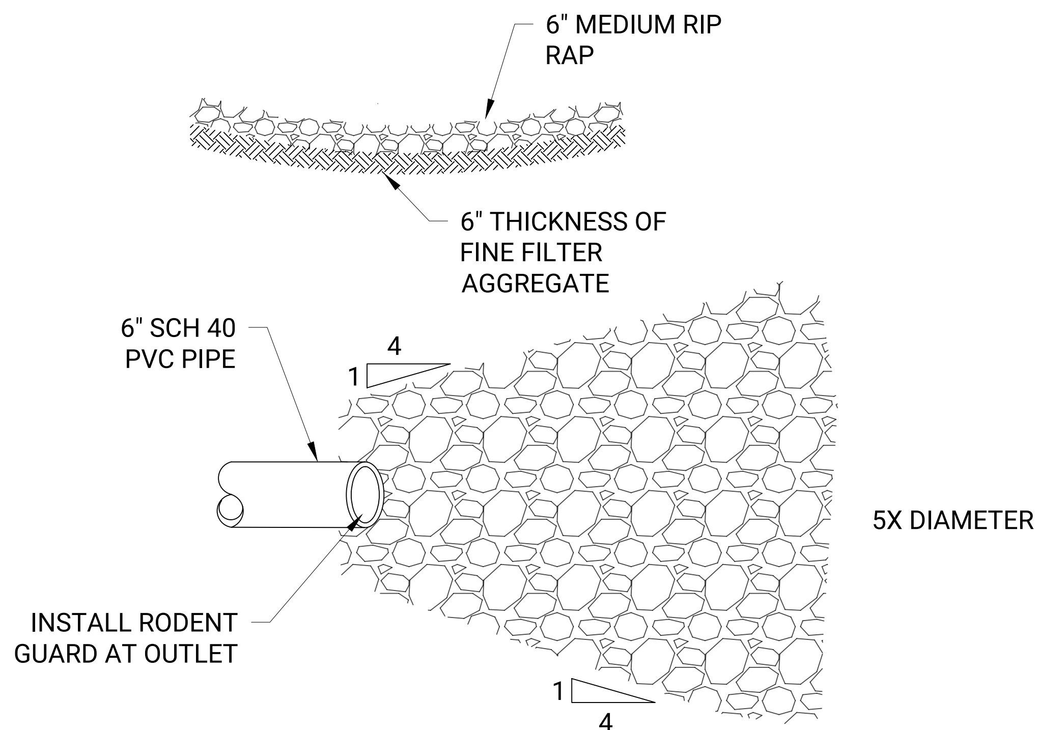
4 PIPE OUTLET PROTECTION C5.1 NOT TO SCALE
