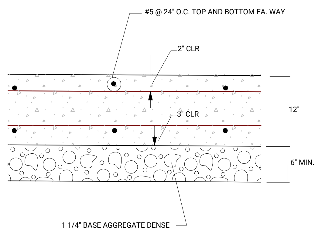
3 TYPICAL CONCRETE PAD DETAIL C5.3 NOT TO SCALE
