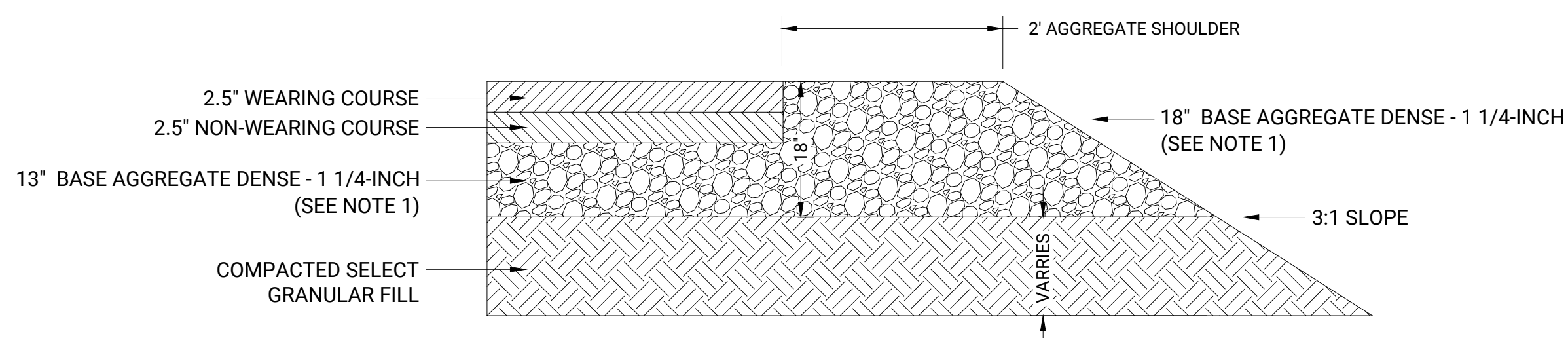
2 AGGREGATE TRANSITION DETAIL C5.1 NOT TO SCALE
