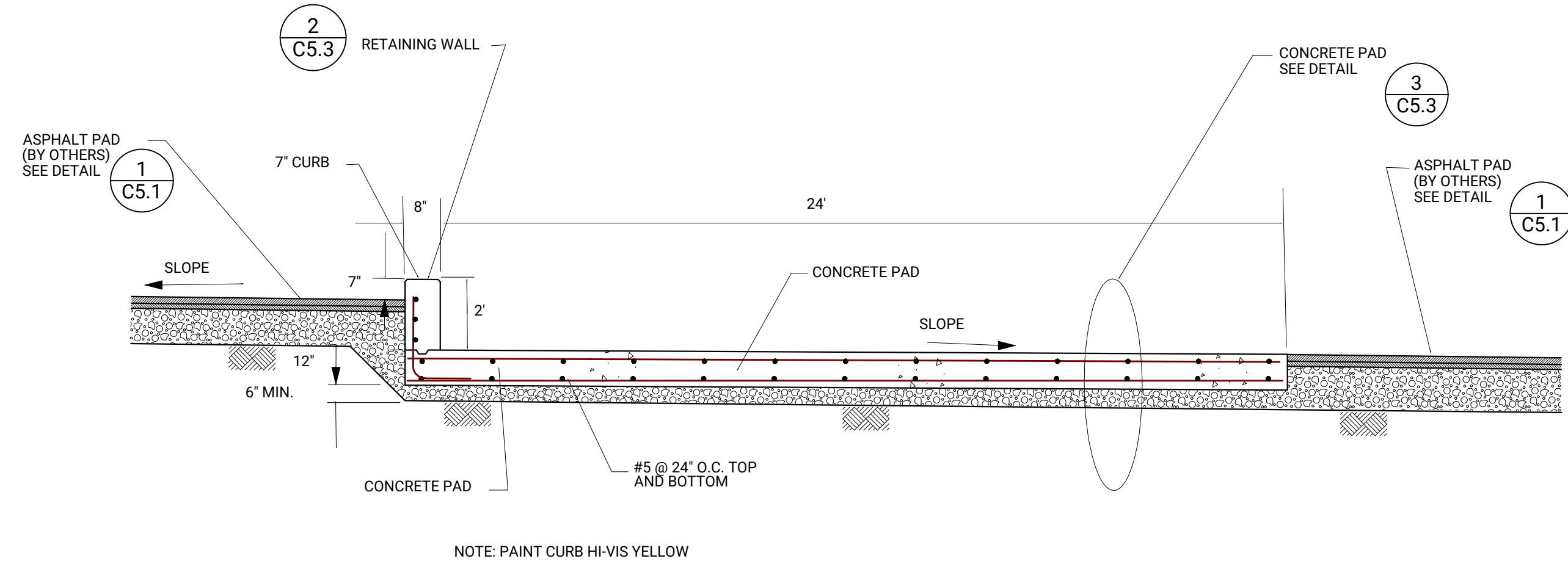
1 TYPICAL SECTION C5.3 NOT TO SCALE
