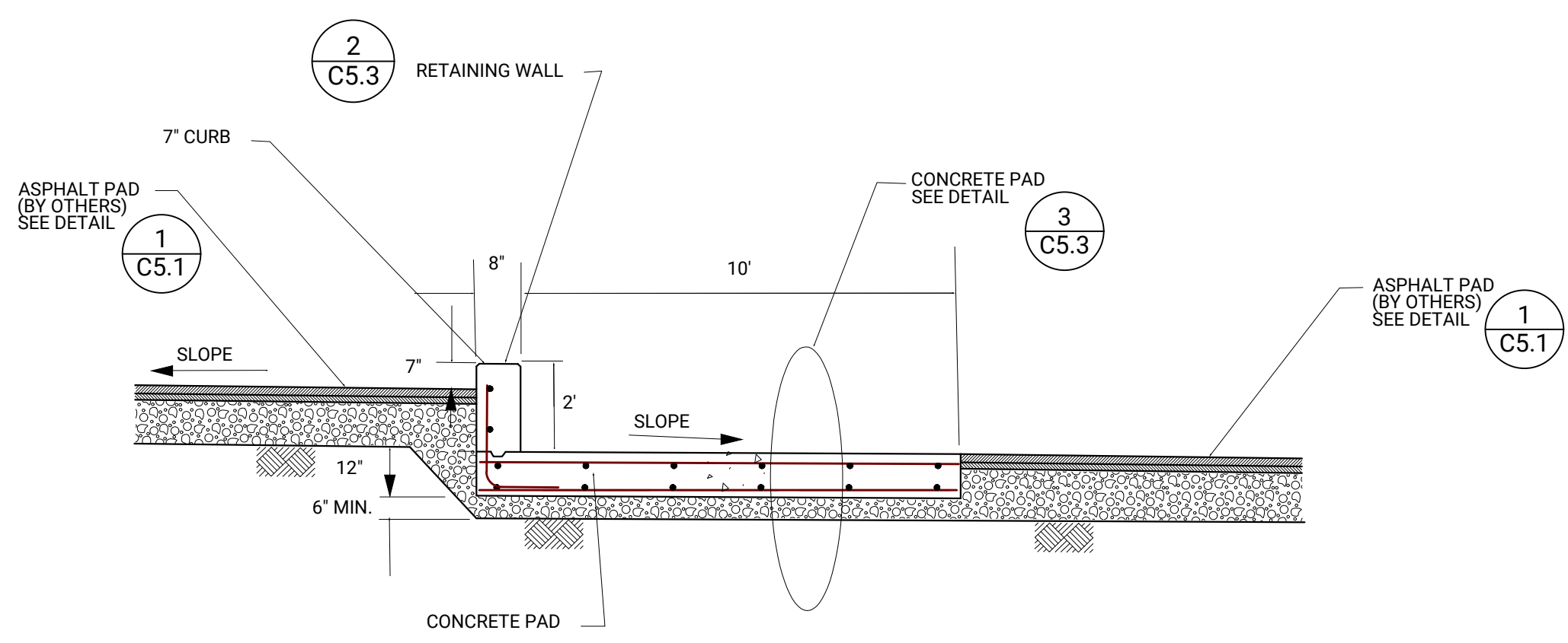
4 TYPICAL SECTION C5.3 NOT TO SCALE
