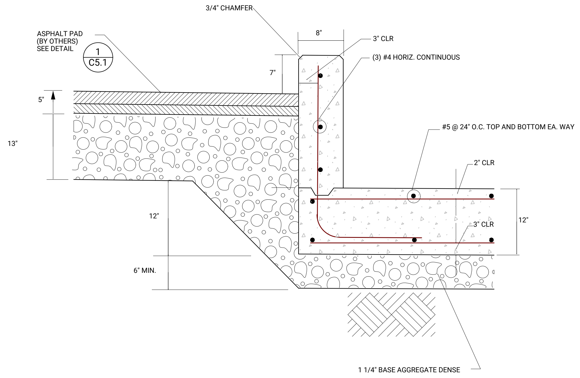
2 TYPICAL RETAINING WALL/CURB SECTION C5.3 NOT TO SCALE
