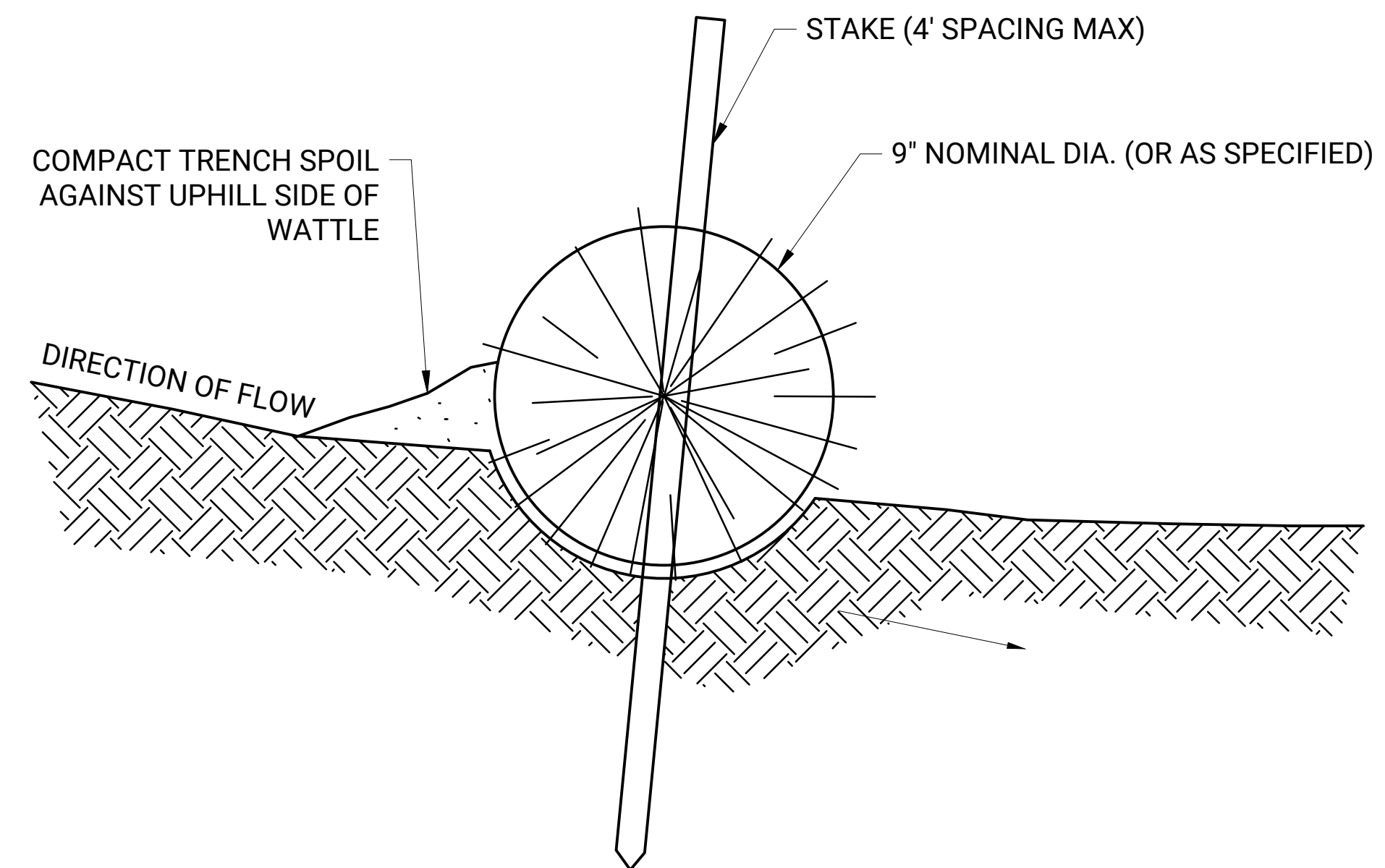
2 STRAW WATTLE SLOPE INTERRUPTION DETAIL C5.0 NOT TO SCALE
