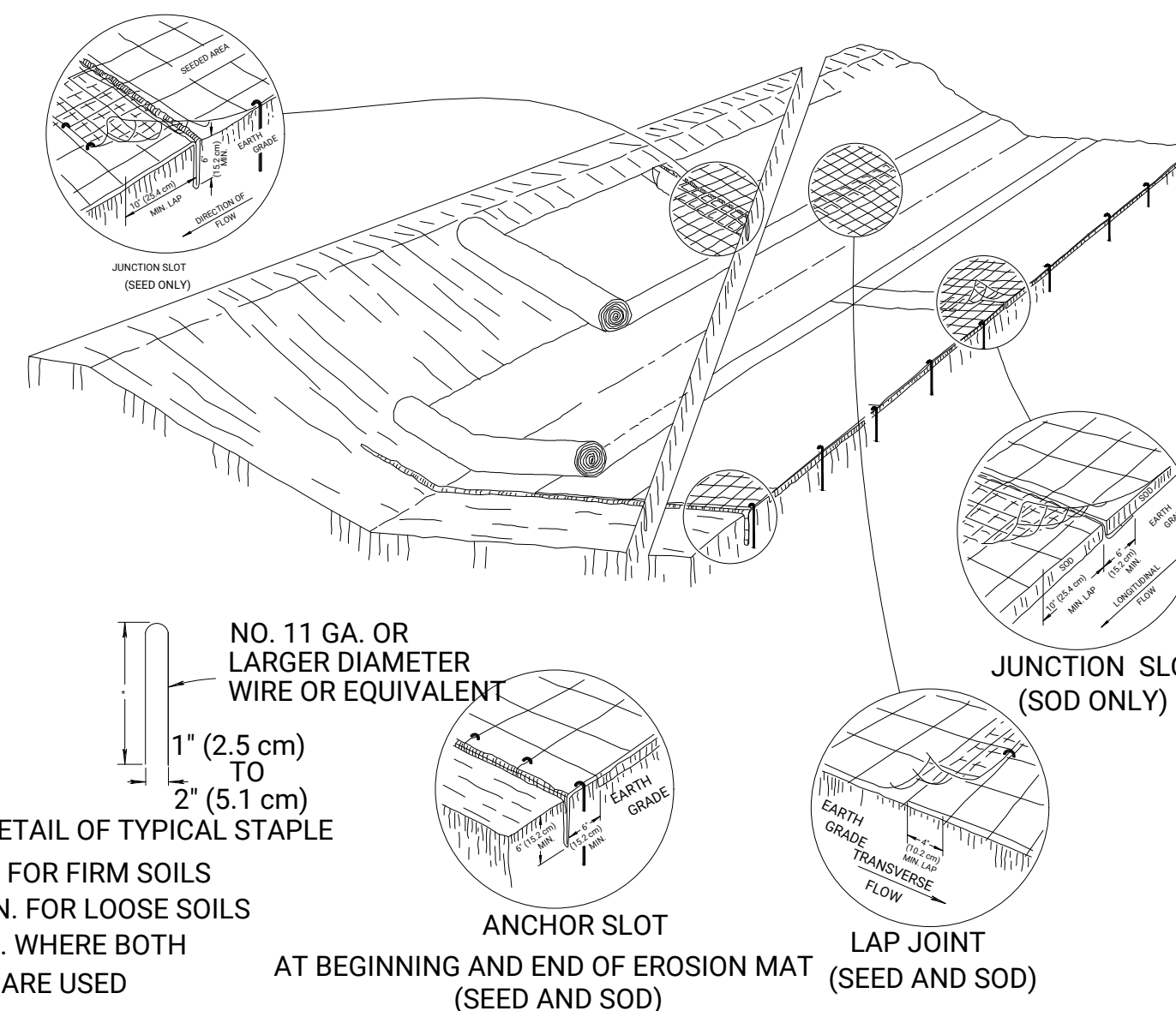
3 EROSION MAT DETAIL C5.0 NOT TO SCALE
