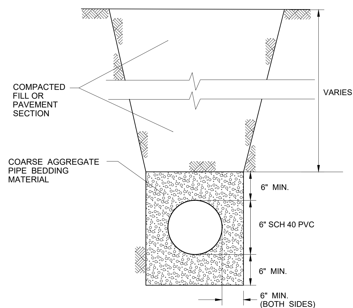
3 PIPE TRENCH DETAIL C5.1 NOT TO SCALE
